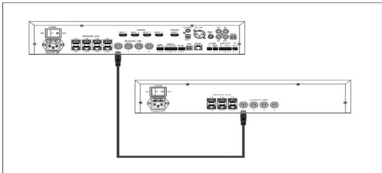
Figure 2.4 The connection of extended controller
