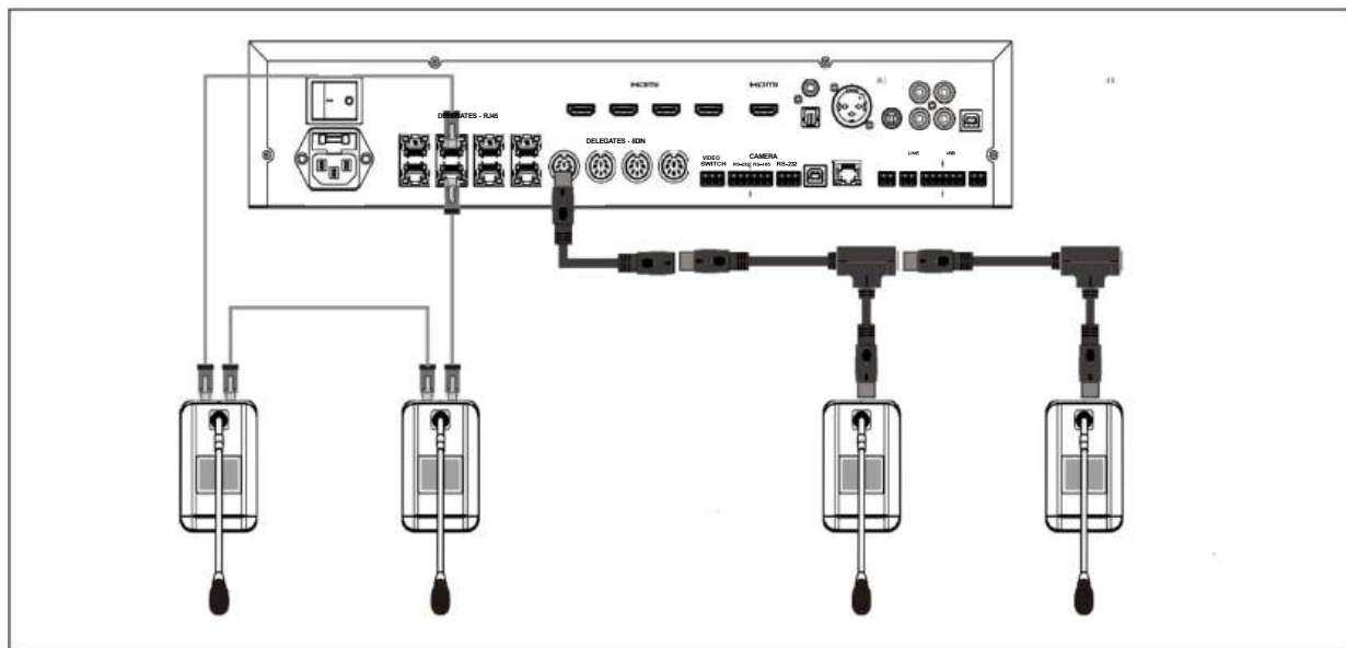
Figure 3.2 The connection between the conference controller and the unit
