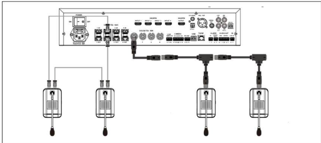
Figure 2.3 The connection between controller and unit
