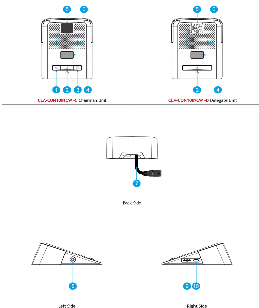
Figure 3.0 Tabletop/Countertop unit
