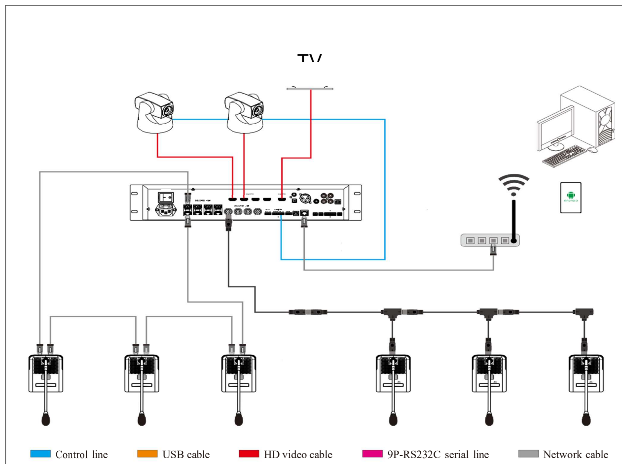
Figure 1.1 System overview
