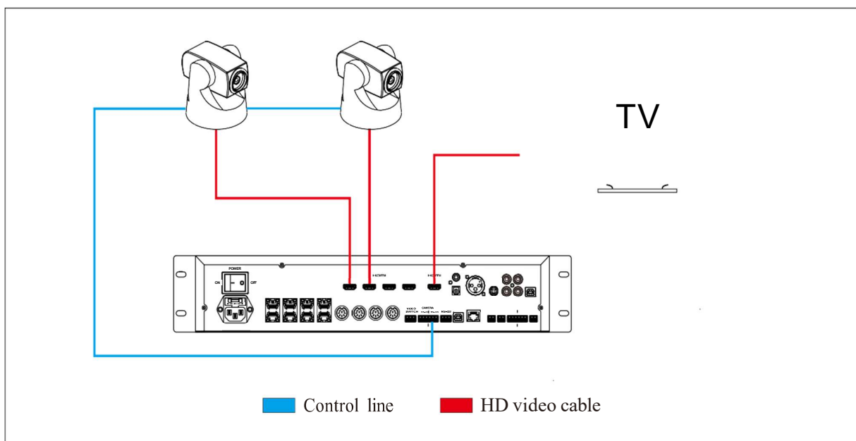
Figure 5.2 Connection with camera
