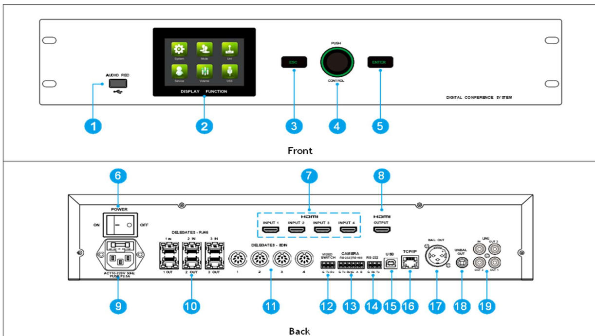
Figure 2.1 Front and rear panels
