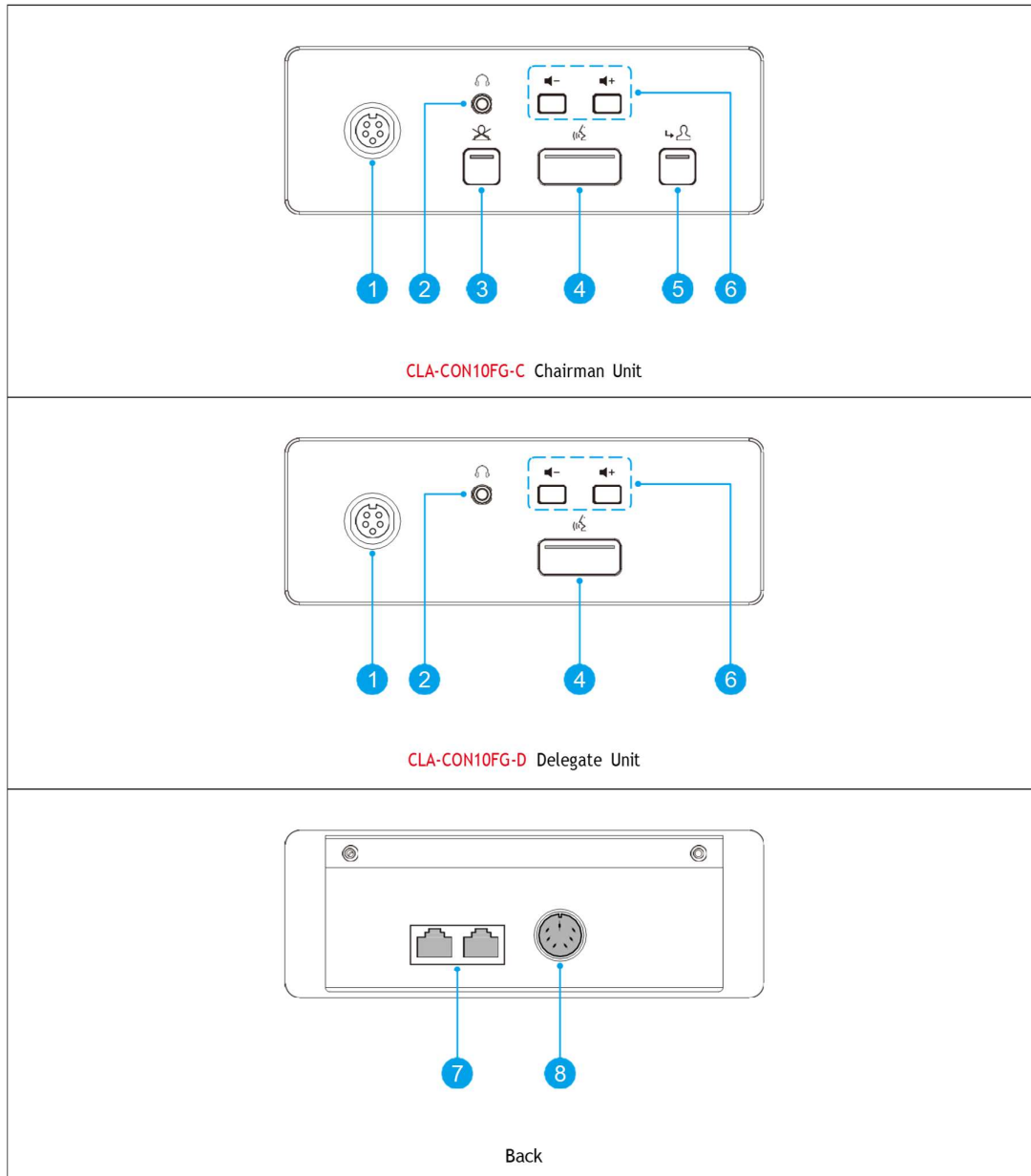
Figure 3.0 Fushmount unit
