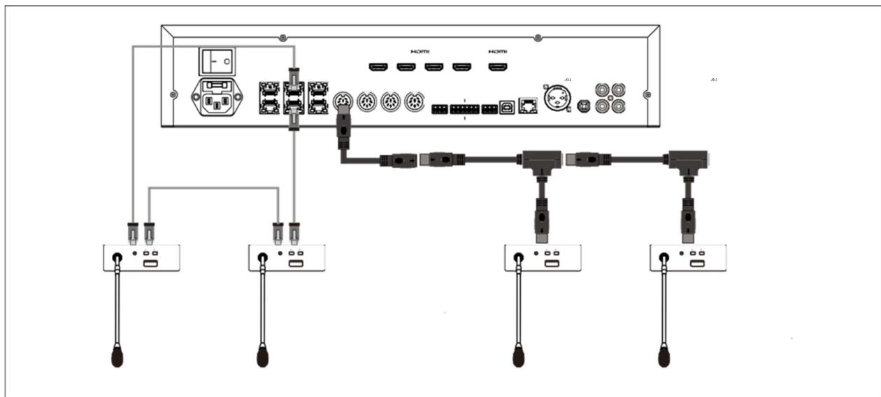
Figure 3.2 The connection between the conference controller and the unit
