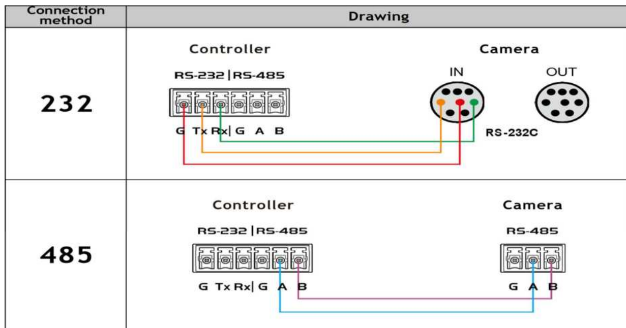
Figure 5.3 Communication connection between the controller and the camera
